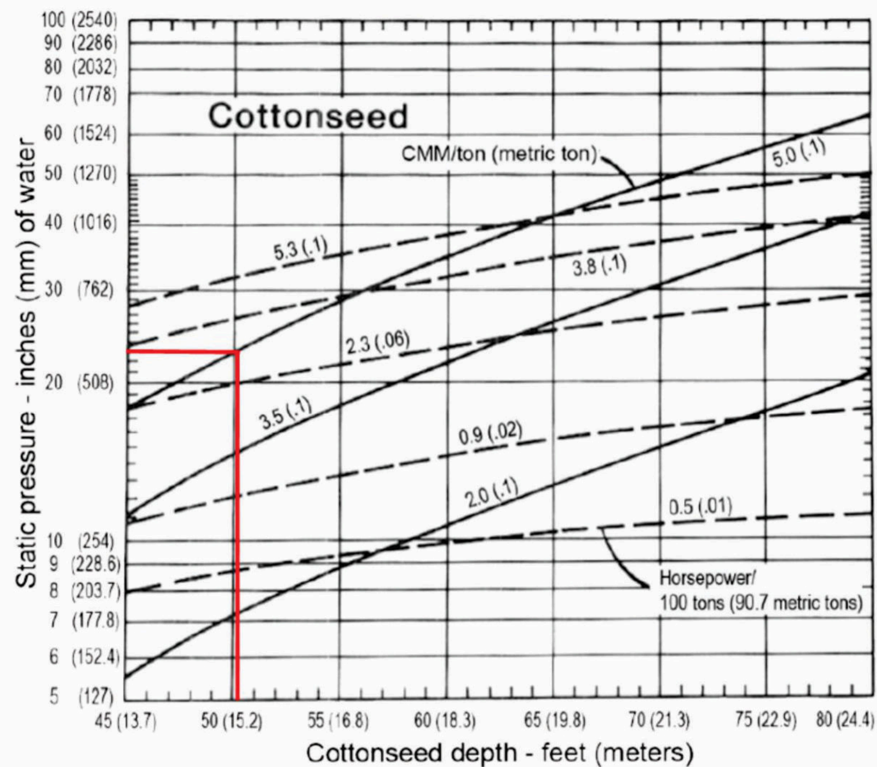
Figure 1. Fan horsepower and static pressure requirements for aerating cottonseed in Muskogee type storage buildings in cubic meters per minute per metric ton (cmm/ton).
